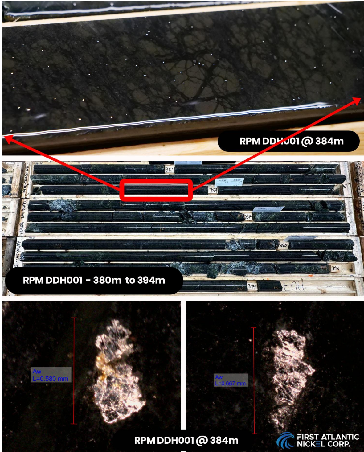
Figure 1: Image showing discovery hole RPM DDH001 (24-AN-02) with disseminated sulfur-free nickel-iron alloy (awaruite). Top image showing close-up of drill core at 384 meters with coarse grained disseminated awaruite; middle image showing core boxes from 380 meters to 394 meters, end of hole; bottom images showing microscope photos of individual large grains of awaruite, 580 microns to 667 microns at 384 meters.
