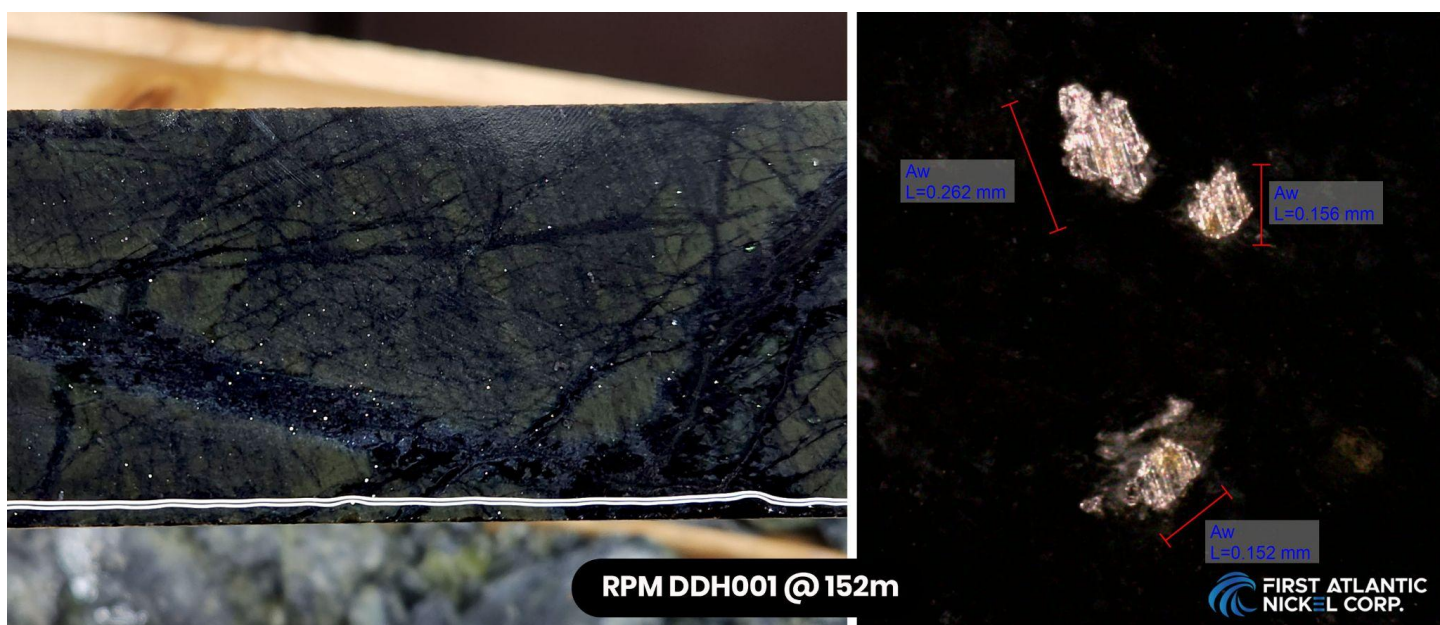
Figure 2: RPM DDH001 (24-AN-02) at 152 meters showing coarse grains of nickel-iron alloy (awaruite). Left image shows drill-core with disseminated awaruite in serpentinized ultramafic cut by serpentine-magnetite fracture fillings and veinlets; Right image shows microscope photo of nickel alloy grains ranging from 152 - 262 microns.
