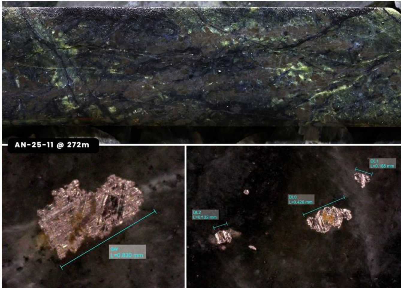
Figure 02: Drill core from Hole AN-25-11 at 272 meters, showing disseminated awaruite (nickel-iron-cobalt alloy) in serpentinized peridotite with magnetite veining (top); photomicrographs show awaruite grains up to ~800 microns in size (bottom).
